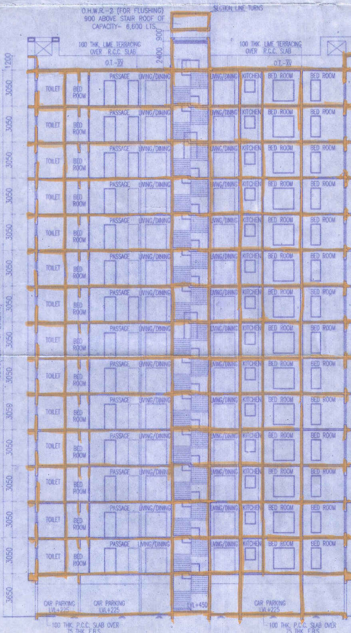
SECTION J-J SIMILAR OF SECTION P-P
